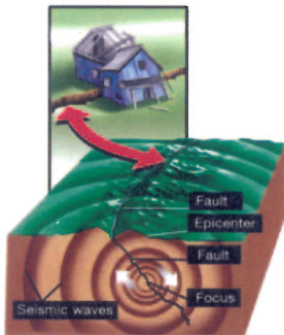
Figure 12.2 The focus, epicenter, and seismic waves of an earthquake occurring at an active fault
